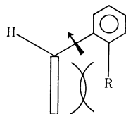
Fig. 2. Molecular deformation of the sp form.
